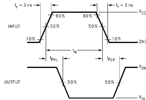
Figure 6. AC Waveforms
