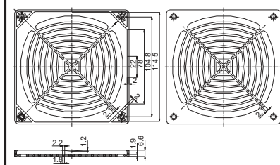
D-1 Finger Guard
