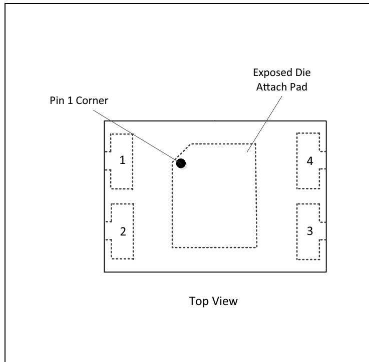
Figure 3: Pin Diagram
