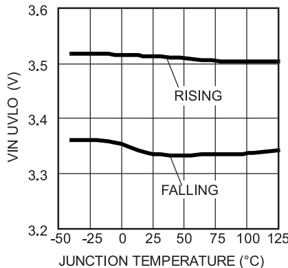
V_{IN} UVLO vs. Junction Temperature
