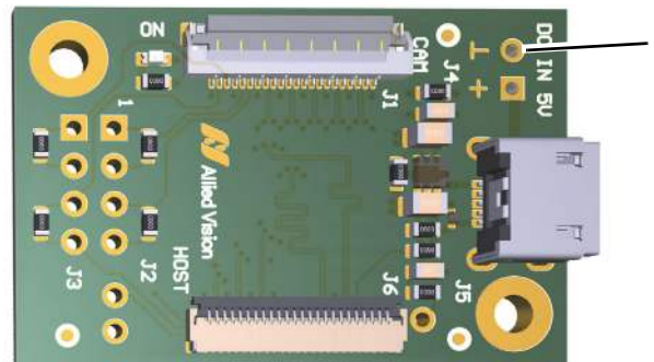
Figure 17: Connecting GND
