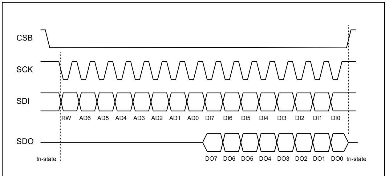
Figure 5: Four wire SPI bit transfer
