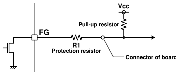
Figure 30. Protection of FG terminal
