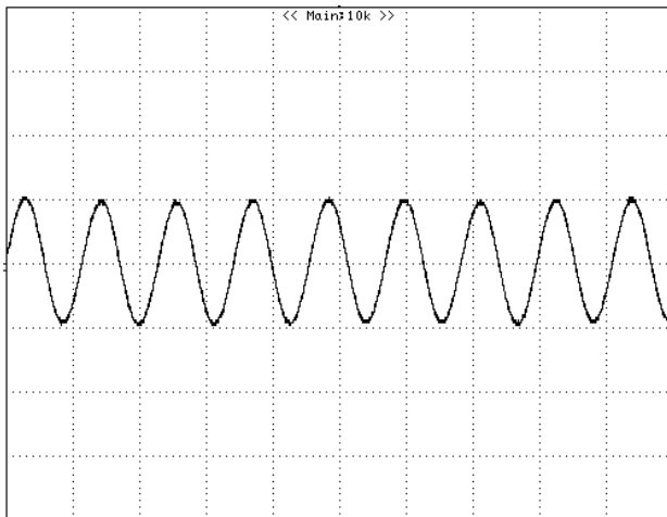
Figure 5: Output ripple & noise at 72Vin, 100% lout CH1:VOUT, 10mV/div, 5uS/div
