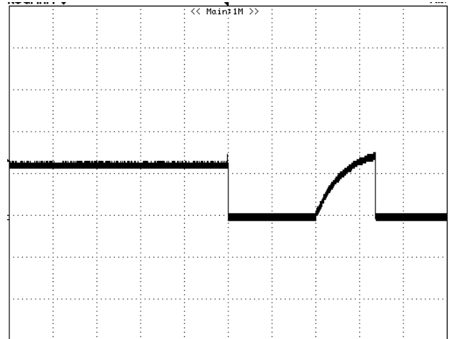
Figure 6: Output over voltage protection at 72Vin, 100% lout CH1:VOUT, 10V/div, 100mS/div
