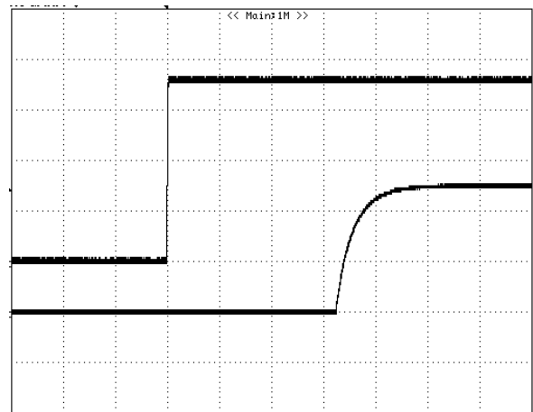
Figure 4: Vout start up with Vin on at 72Vin, 100% lout, TOP:VIN, 20V/div, 200mS/div BOTTOM: VOUT, 5V/div, 200mS/div
