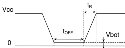
Figure 60. Rise waveform
