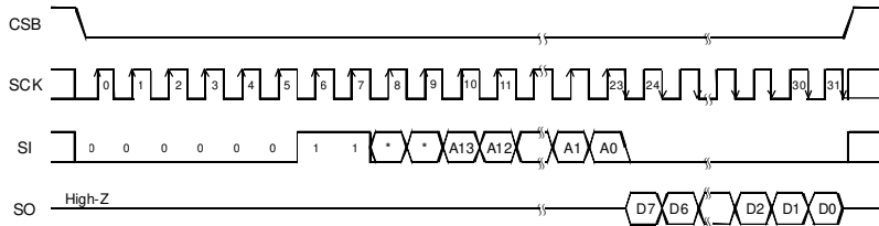
Figure 39. Read command
