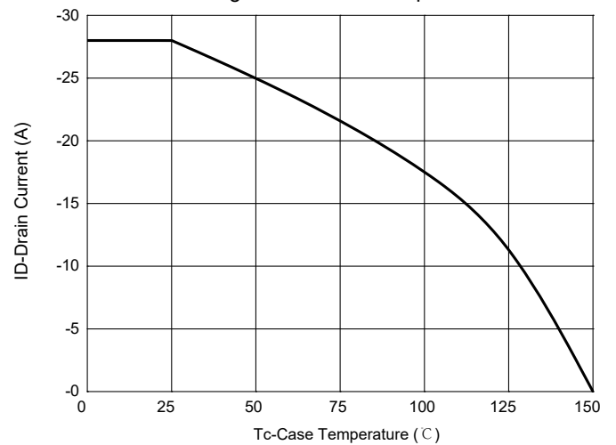
Fig. 10 - Current dissipation
