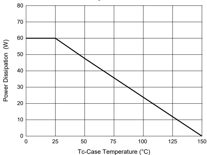
Fig.11-PD-TC
