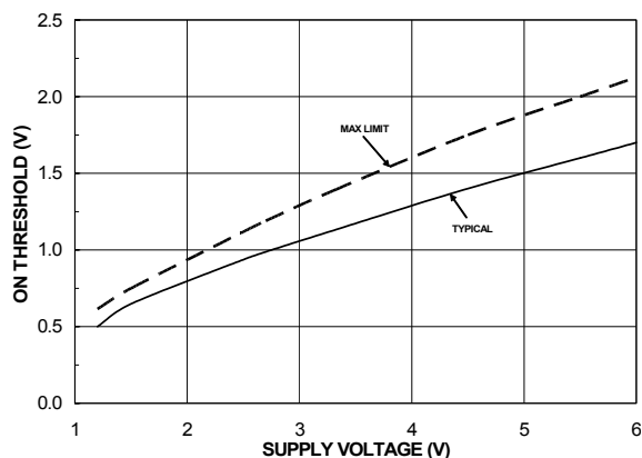
Figure 2. ON Threshold vs. V_{IN}
