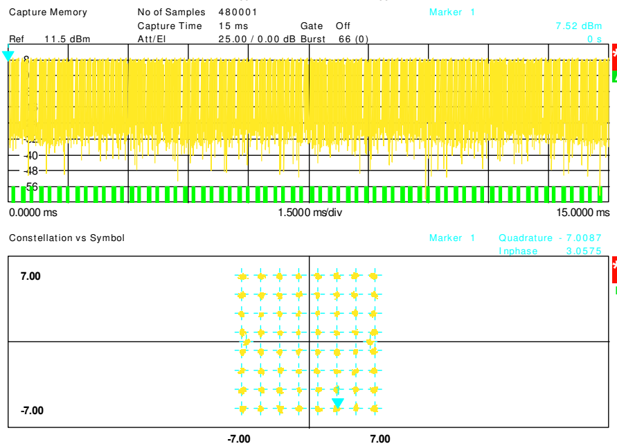
Figure 7 WiMax constellation Pavg= 25.8 dBm at 5.9 GHz. for 2.5% EVM.
