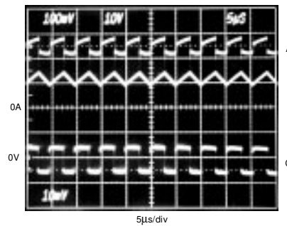
CIRCUIT OF FIGURE 2, V+ = 5V, V OUT = -5V, I LOAD = 240mA A: OUTPUT RIPPLE, 100mV/div B: INDUCTOR CURRENT, 50mA/div C: LX WAVEFORM, 10V/div
