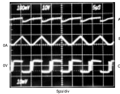
CIRCUIT OF FIGURE 2, V+ = 5V, V OUT = -5V, I LOAD = 80mA A: OUTPUT RIPPLE, 100mV/div B: INDUCTOR CURRENT, 50mA/div C: LX WAVEFORM, 10V/div
