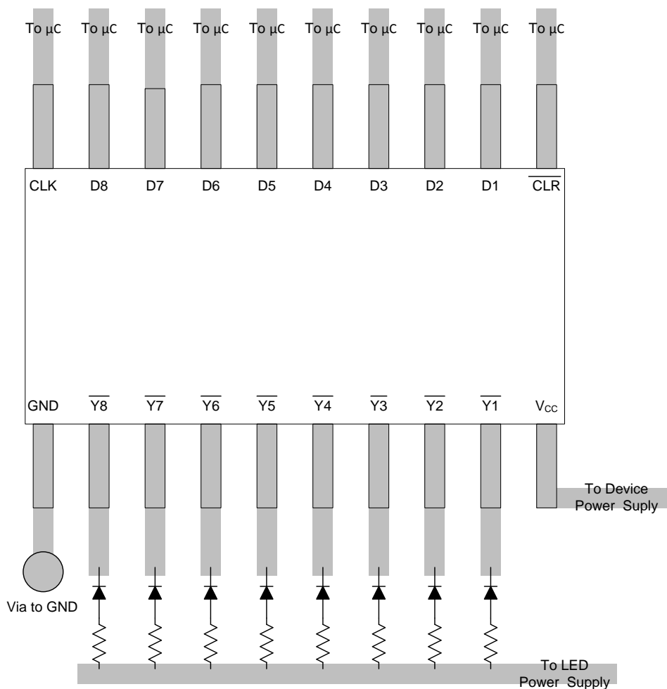
Figure 11. Layout Example
