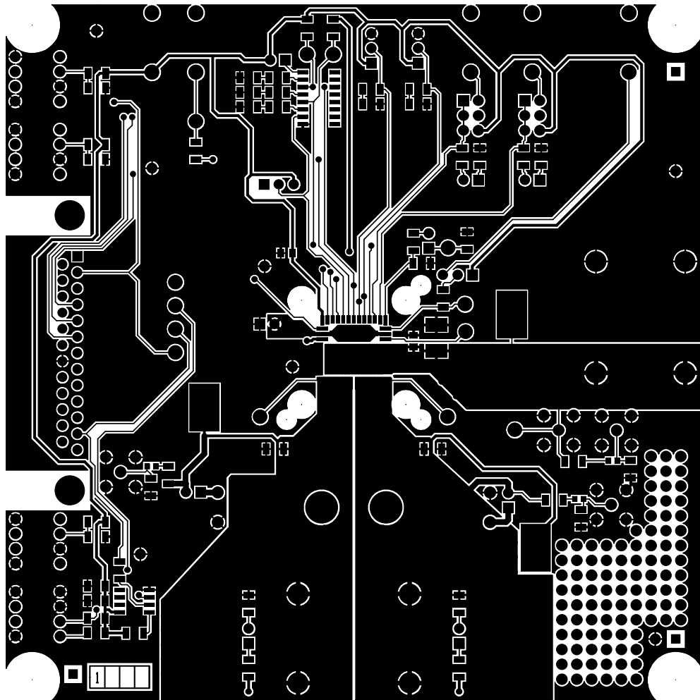
Figure 8. KIT10XS4200EVBE Assembly Layer Top
