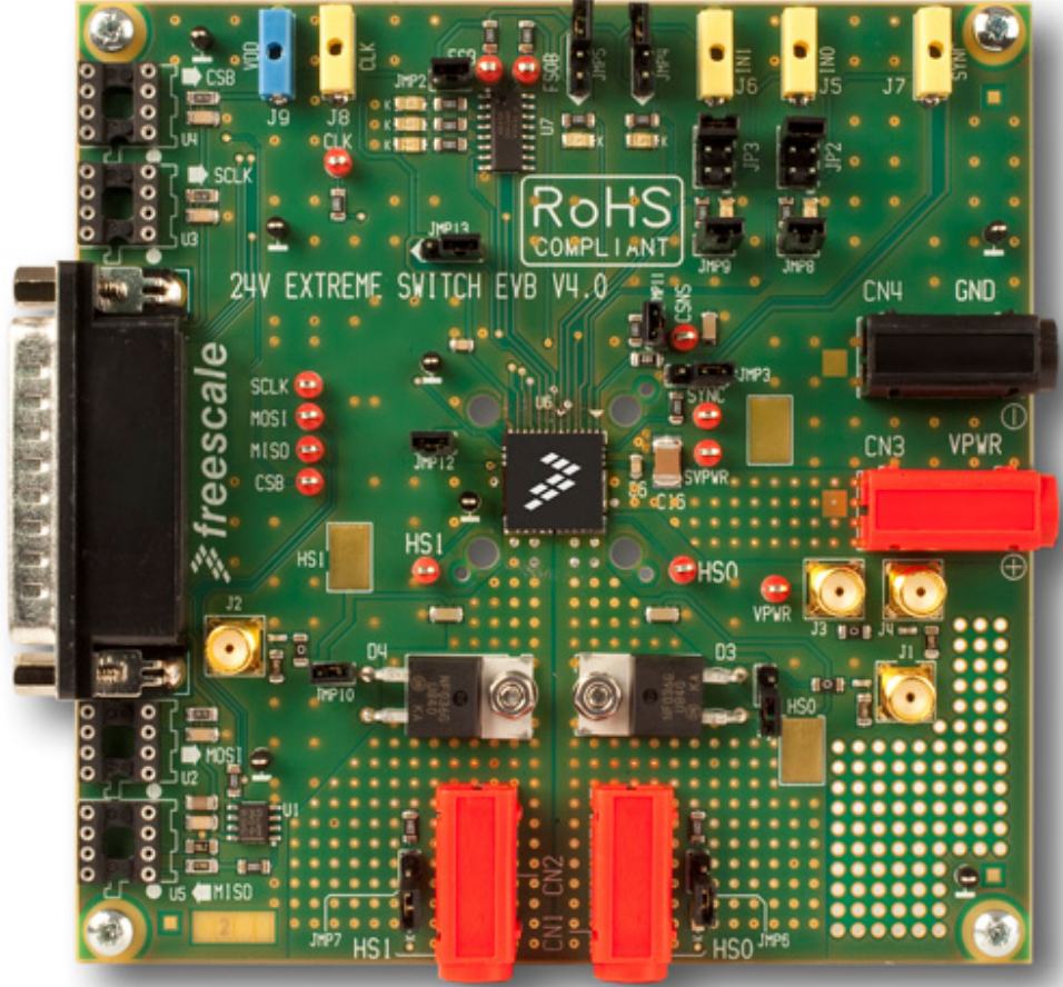
Figure 1. KIT10XS4200EVBE Evaluation Board
