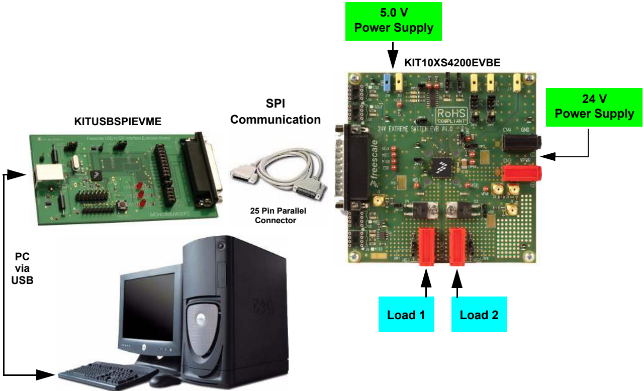
Figure 2. KIT10XS4200 Setup Configuration Diagram
