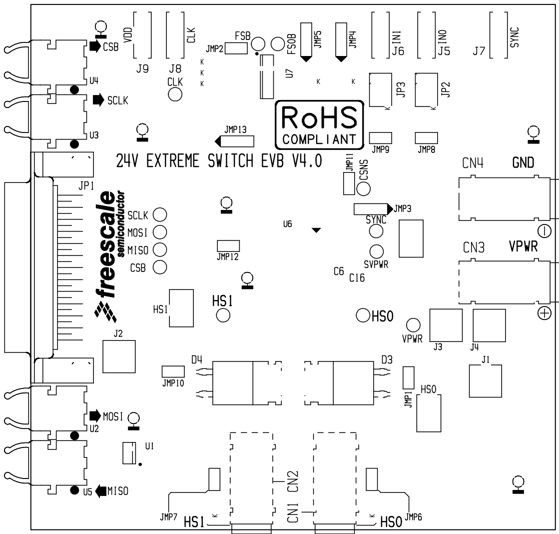
Figure 10. KIT10XS4200EVBE Silkscreen
