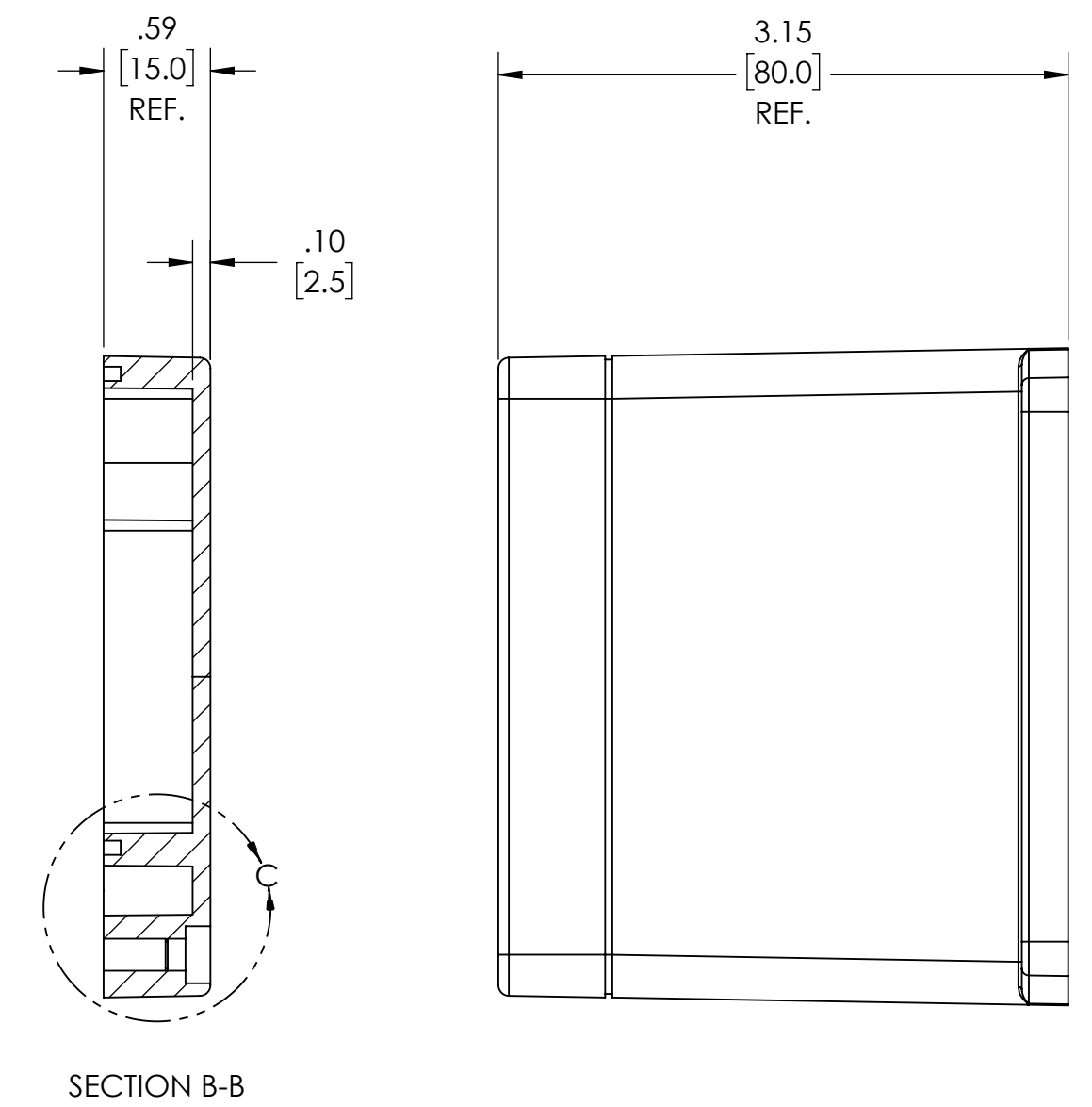
SECTION B-B
