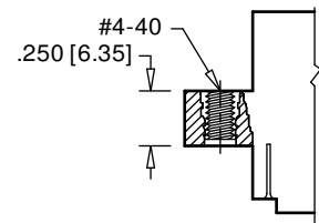
THREADED INSERT (T)
