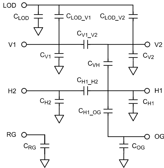
Figure 10. Equivalent Circuit Model
