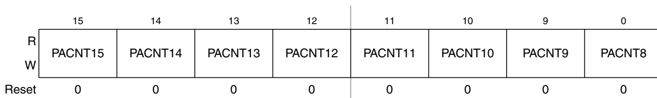
Figure 22-26. Pulse Accumulator Count Register High (PACNTH)
