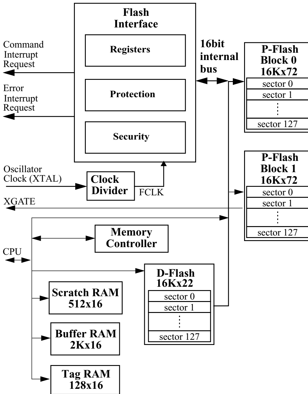
Figure 25-1. FTM256K2 Block Diagram
