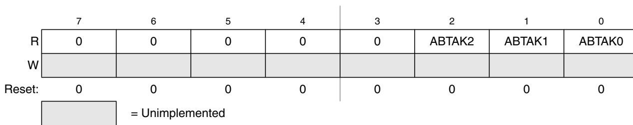
Figure 16-13. MSCAN Transmitter Message Abort Acknowledge Register (CANTAANK)
