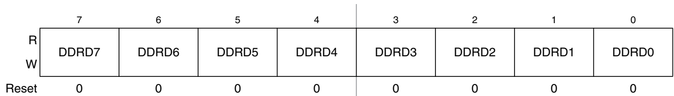
Figure 2-8. Port D Data Direction Register (DDRD)
