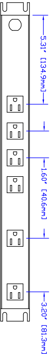
BOTTOM VIEW
