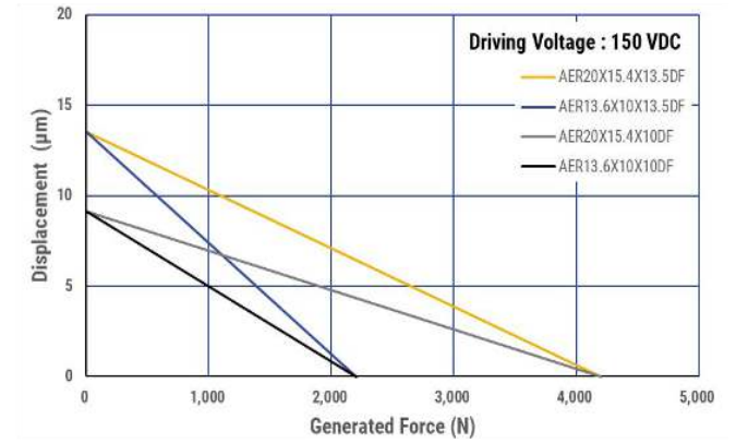
Figure 2 - Generated Force vs. Displacement
