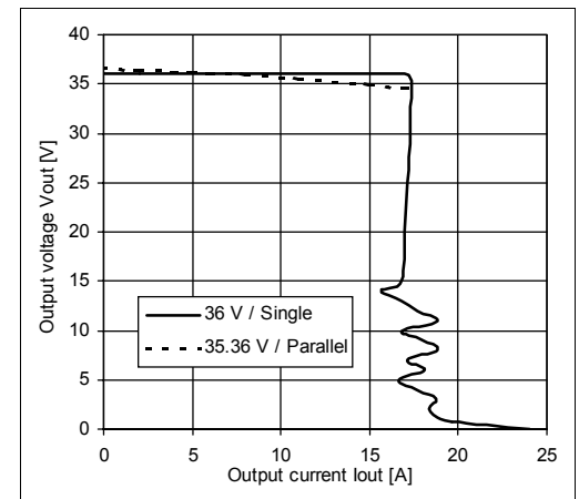
Output characteristic (typ.)
