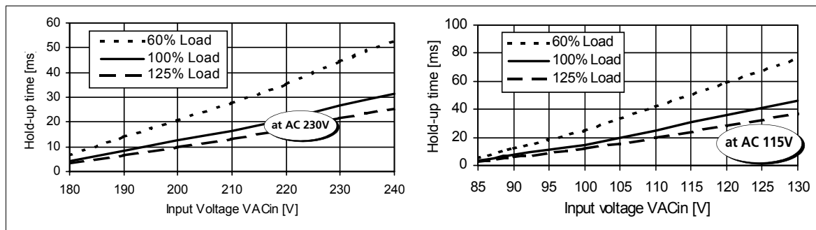
Hold-up time (min., at V_{out}=36\text{V} )
