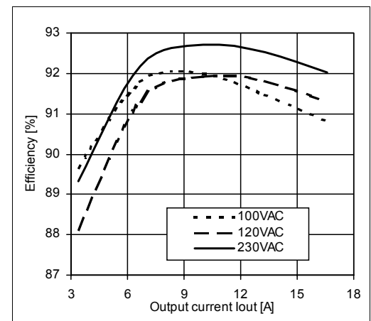
Efficiency (typ., at V_{out}=36\text{V} )
