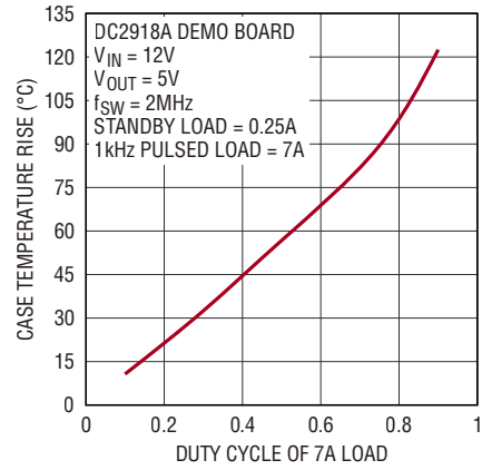
Figure 3. Temperature Rising vs Input Voltage
