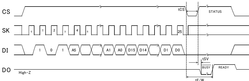
Figure 31. Write Cycle
