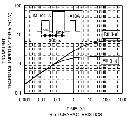
R_{\theta-t} CHARACTERISTICS
