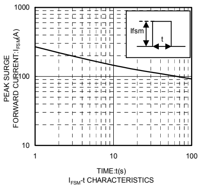
I_{FSM} \cdot t CHARACTERISTICS
