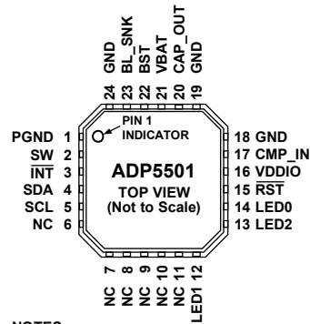
Figure 3. Pin Configuration
