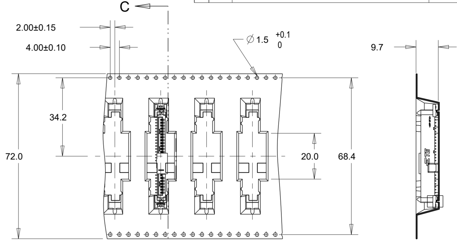
SECTION C-C
