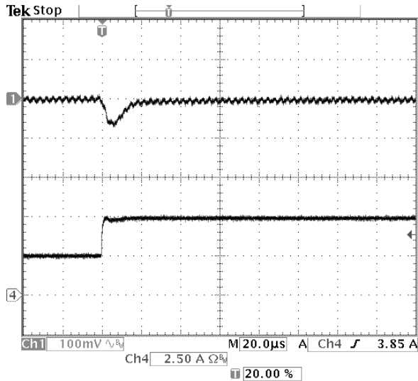
Fig-1.0V-6: Output voltage response for V_{out}=1.0V to positive load current step-change from 2.5A to 5A with slew rate of 5A/\mu s at V_{in}=5.0V . C_o=47\mu F \times 2 ceramic. Top trace: output voltage (100mV/div.) Bottom trace: load current (2.5A/div.) Time scale: 20μs/div.
