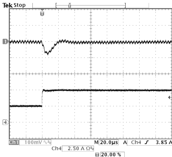
Fig-1.8V-6: Output voltage response for V_{out}=1.8V to positive load current step-change from 2.5A to 5A with slew rate of 5A/\mu s at V_{in}=5.0V . C_o=47\mu F \times 2 ceramic. Top trace: output voltage (100mV/div.) Bottom trace: load current (2.5A/div.) Time scale: 20μs/div.
