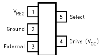
Figure 1. 5-Lead SOT23-5 Surface Mount Package See Package MF05A
