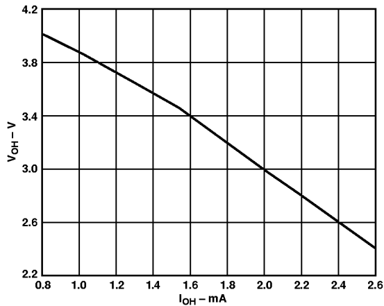
Figure 27. Source Capability of Status Output (ADDC02805SA)
