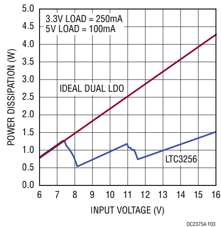
Figure 3. Power Dissipation vs Input Voltage
