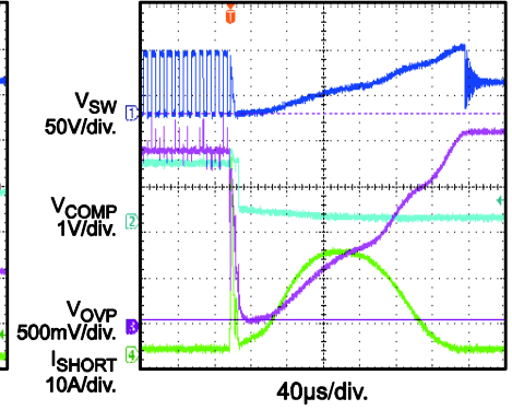
Short to GND
