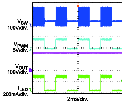
PWM Dimming f_{PWM}=200\text{Hz}
