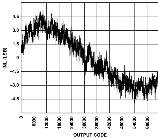
Figure 37. INL, f_{IN} = 9.7 MHz, f_{SAMPLE} = 125 MSPS, V_{REF} = 1.3 V
