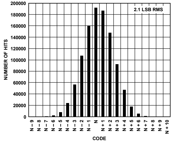
Figure 39. Input-Referred Noise Histogram, f_{SAMPLE} = 125 MSPS, V_{REF} = 1.3 V
