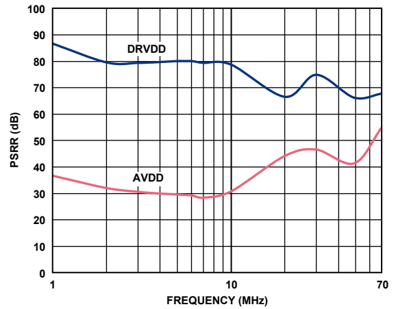
Figure 40. PSRR vs. Frequency, f_{SAMPLE} = 125 MSPS, V_{REF} = 1.3 V
