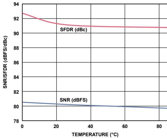
Figure 36. SNR/SFDR vs. Temperature, f_{IN} = 9.7 MHz, f_{SAMPLE} = 125 MSPS, V_{REF} = 1.3 V
