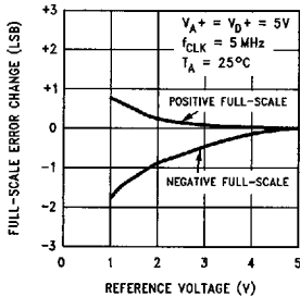
Full-Scale Error Change vs Reference Voltage
