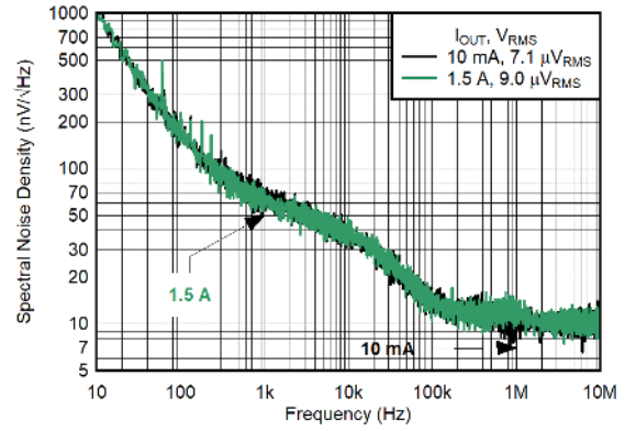
Figure 6-8. Noise vs Frequency and I_{OUT} for V_{OUT} = 0.65\text{ V}
