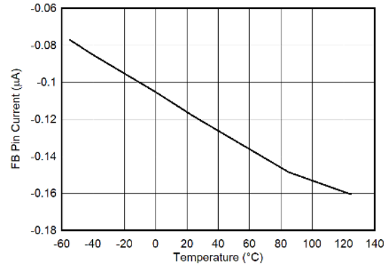
Figure 6-50. FB Pin Current vs Temperature
