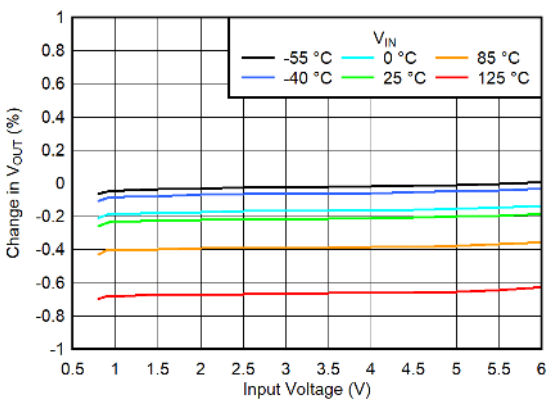
C_{IN} = C_{OUT} = 10\ \mu\text{F} , C_{BIAS} = 1\ \mu\text{F} , C_{SS} = 0\text{ nF} , V_{BIAS} = 5\text{ V} , V_{EN} = 1.1\text{ V}
