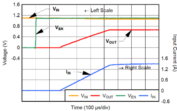
C_{IN} = C_{OUT} = 10\ \mu\text{F} , C_{BIAS} = 1\ \mu\text{F} , I_{OUT} = 1.5\text{ A} , V_{IN} = 1.1\text{ V} , V_{BIAS} = 5\text{ V}
