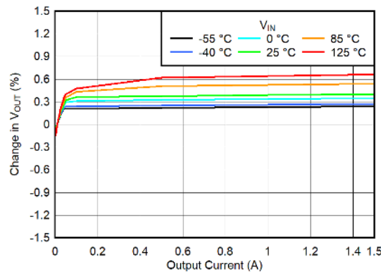
Figure 6-28. Load Regulation for I_{OUT} = 0\text{ A} to Load, V_{OUT} = 0.65\text{ V}
