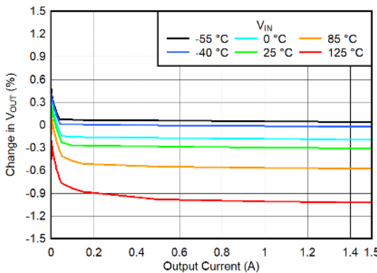
Figure 6-29. Load Regulation for I_{OUT} = 0\text{ A} to Load, V_{OUT} = 3.3\text{ V}
