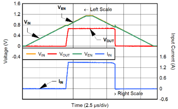
C_{IN} = C_{OUT} = 10\ \mu\text{F} , C_{BIAS} = 1\ \mu\text{F} , I_{OUT} = 1.5\text{ A} , V_{BIAS} = 5\text{ V}
