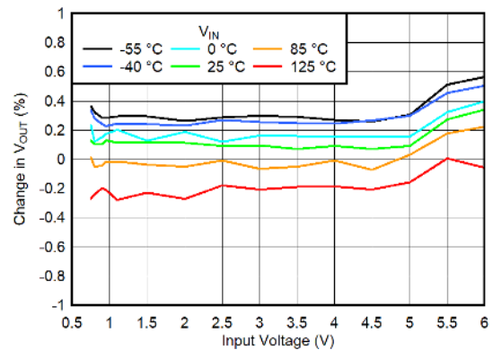
C_{IN} = C_{OUT} = 10\ \mu\text{F} , C_{BIAS} = 1\ \mu\text{F} , C_{SS} = 0\text{ nF} , V_{BIAS} = 5\text{ V} , V_{EN} = 1.1\text{ V}
