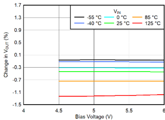
Figure 6-25. BIAS Line Regulation for V_{OUT} = 3.3\text{ V} , I_{OUT} = 0\text{ A}
