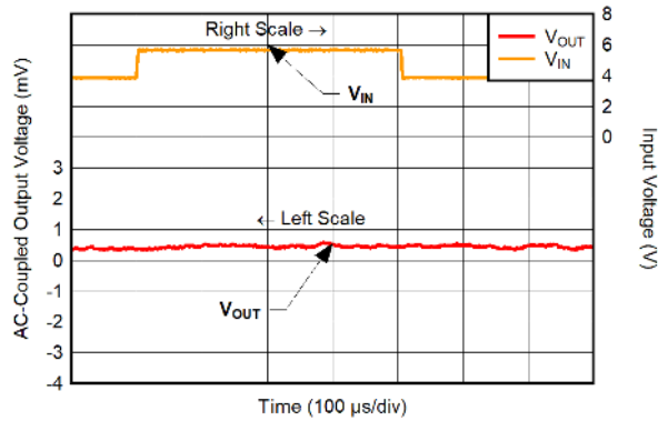
C_{IN} = C_{OUT} = 10\ \mu\text{F} , C_{BIAS} = 1\ \mu\text{F} , I_{OUT} = 1.5\text{ A} , V_{IN} = 3.9\text{ V to } 5.8\text{ V to } 3.9\text{ V at } 1\text{ V}/\mu\text{s}
