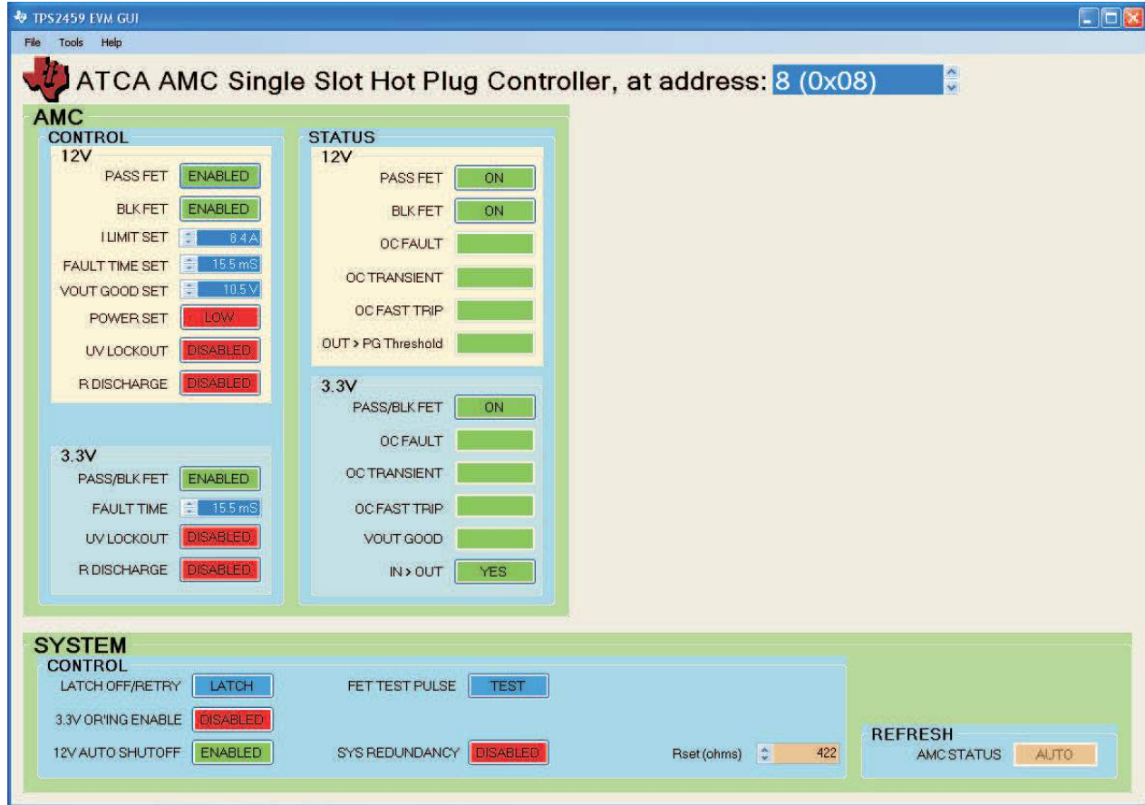
Figure 7. TPS2459 EVM GUI Display – Both Channels Successfully Powered
