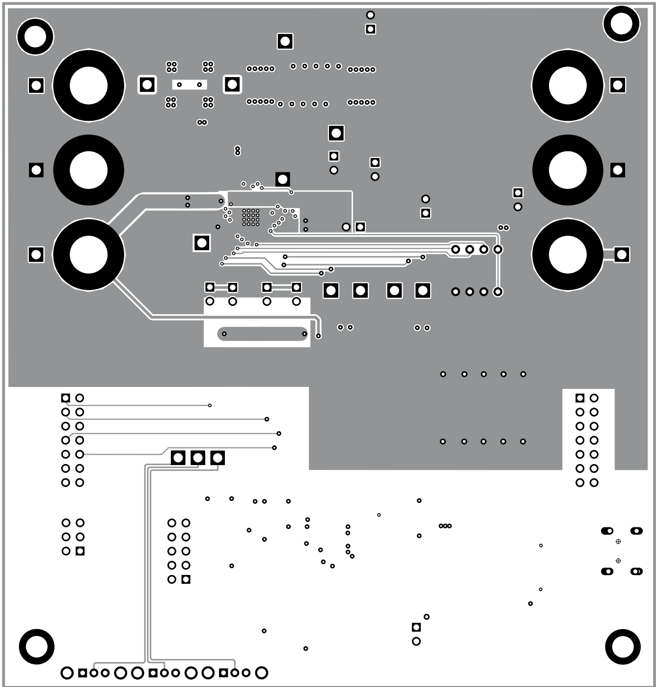
Figure 10. Layer 2 Routing
