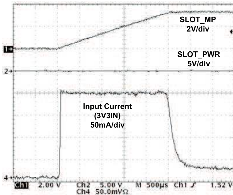
Figure 5. Output Ramp-Up waveforms - SLOT_MP Rail.
