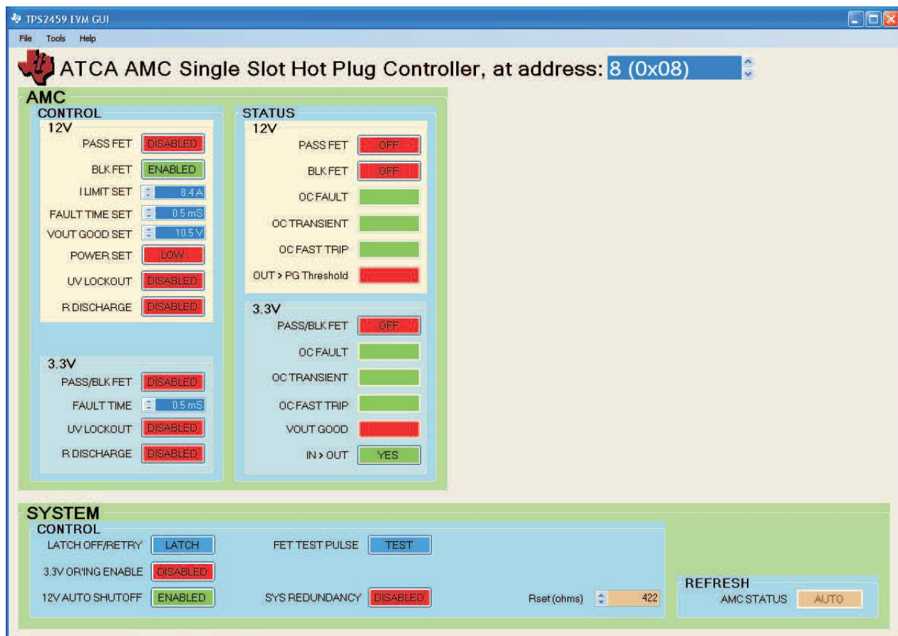
Figure 4. GUI Initial Control and Status Display at Launch
