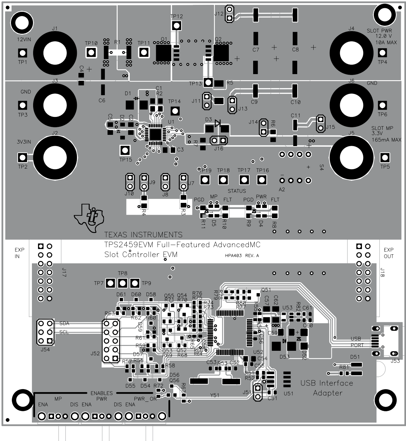
Figure 8. Top Assembly
