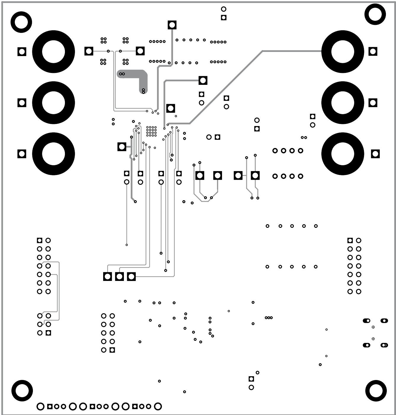
Figure 11. Layer 3 Routing
