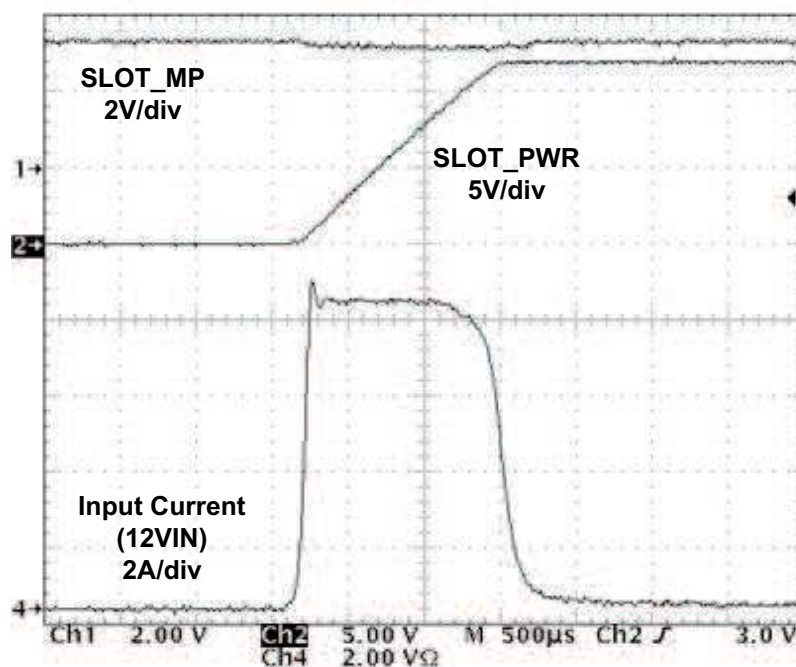
Figure 6. Output Ramp-Up Waveforms - SLOT_PWR Rail.
