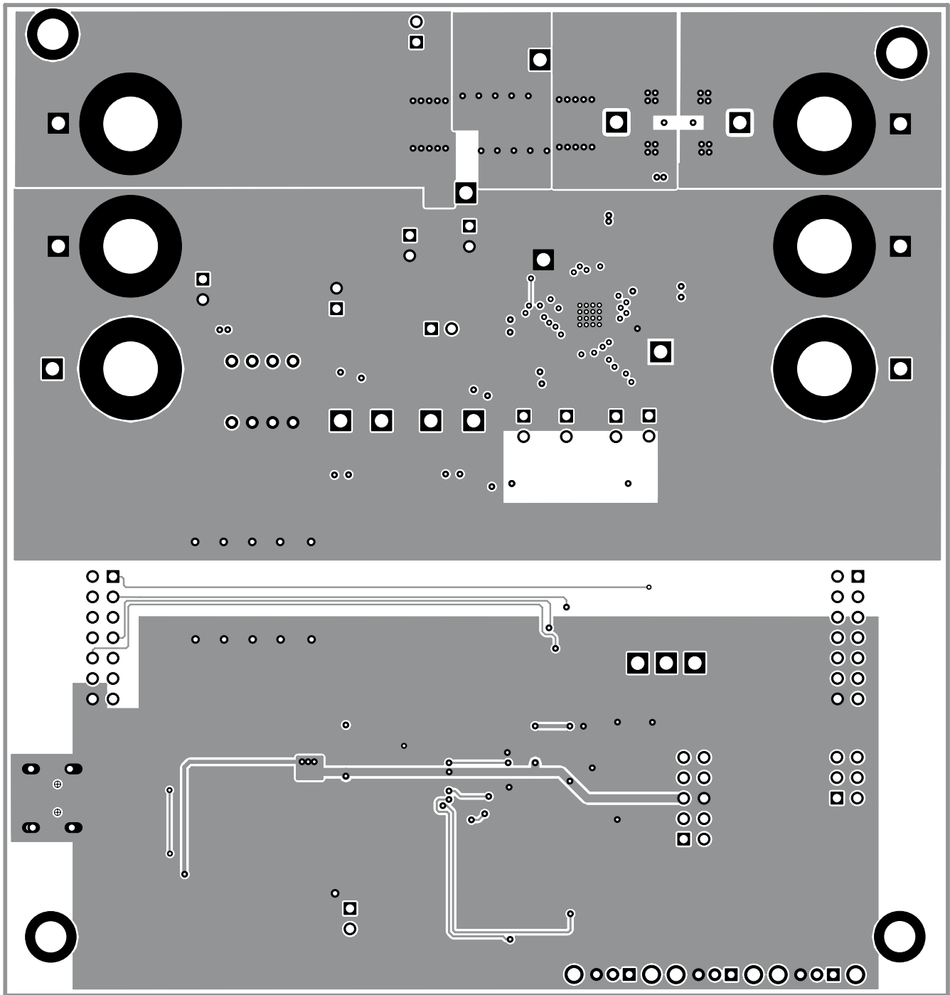
Figure 12. Bottom Layer Routing
