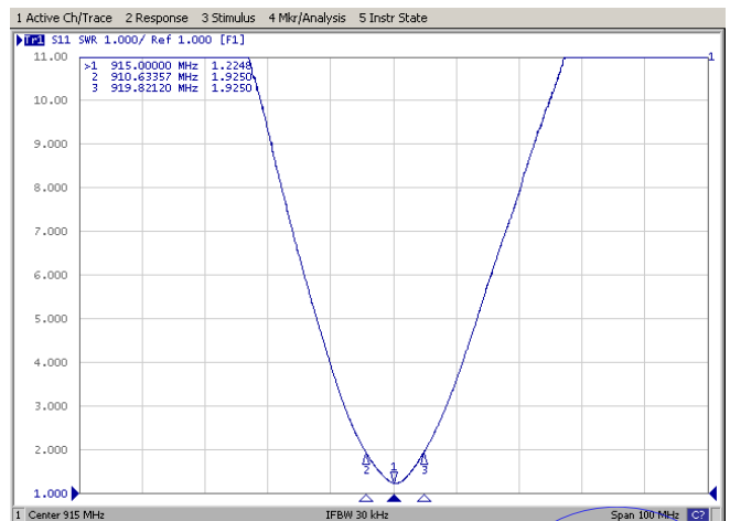
VSWR ( S_{11} )
