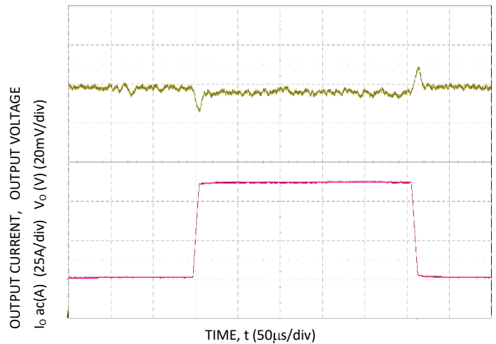
Figure 10. Trans. Resp. to 10A/µs Load Change from 25% to 75% at 12V IN . C_o=4 \times 0.047\mu\text{F} + 4 \times 0.1\mu\text{F} + 15 \times 22\mu\text{F} + 73 \times 47\mu\text{F} + 6 \times 470\mu\text{F} polymer
