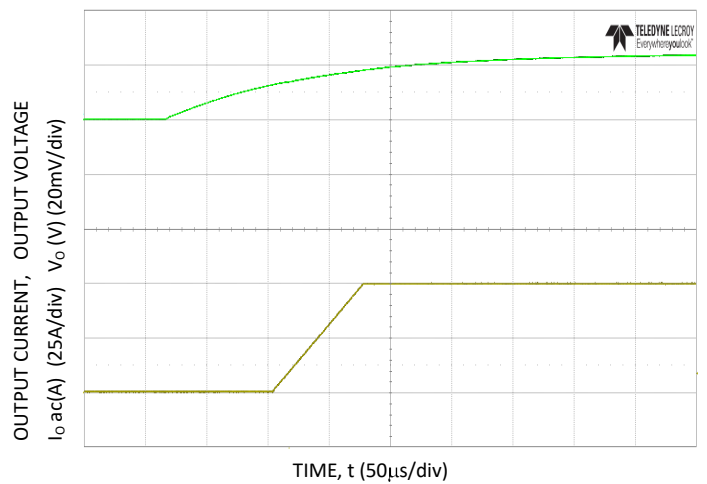
Figure 22. Trans. Resp. to 10\text{A}/\mu\text{s} Load Change from 25% to 75% at 12\text{V}_{IN} , C_o=4 \times 0.047\mu\text{F} + 4 \times 0.1\mu\text{F} + 15 \times 22\mu\text{F} + 73 \times 47\mu\text{F} + 6 \times 470\mu\text{F} polymer
