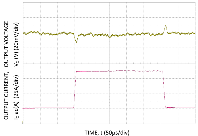
Figure 4. Trans. Resp. to 10A/ \mu\text{s} Load Change from 25% to 75% at 12VIN, C_o=4 \times 0.047\mu\text{F} + 4 \times 0.1\mu\text{F} + 15 \times 22\mu\text{F} + 73 \times 47\mu\text{F} + 6 \times 470\mu\text{F} polymer
