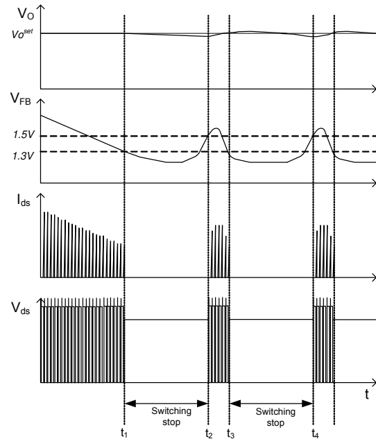
Figure 25. Burst-Mode Operation
