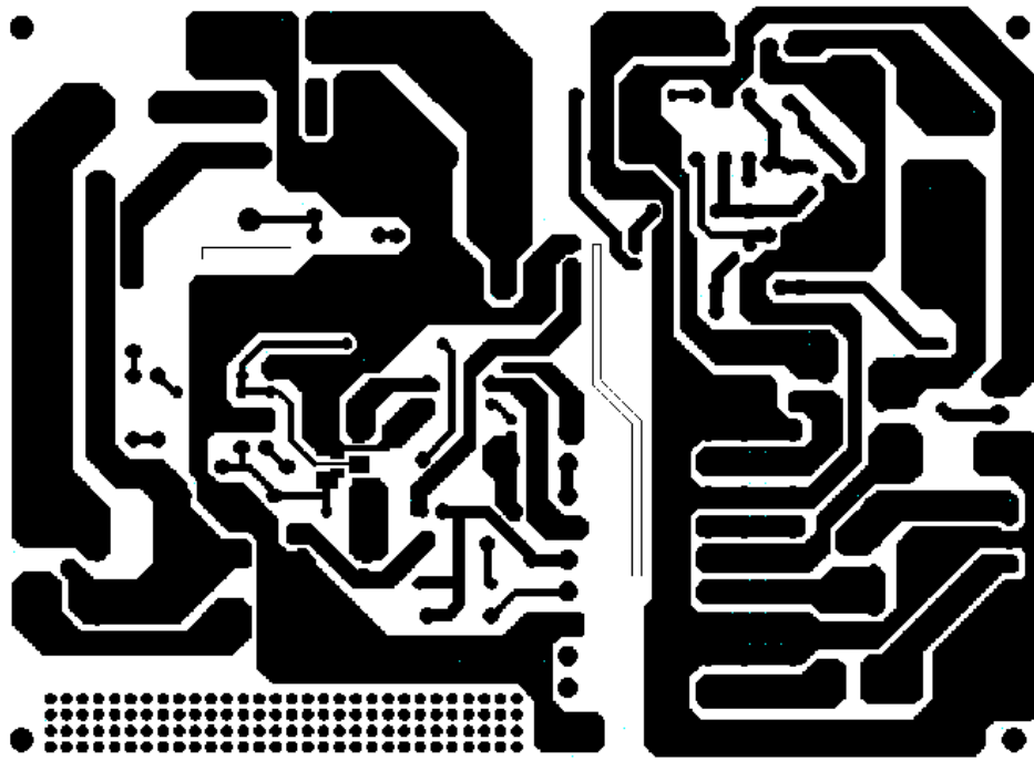
Figure 48. Bottom View
