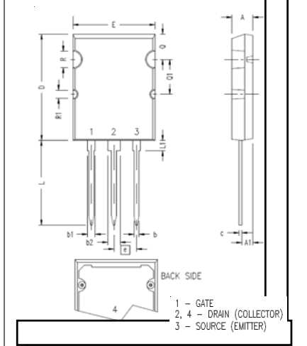
PLUS264™ (IXTB) Outline
