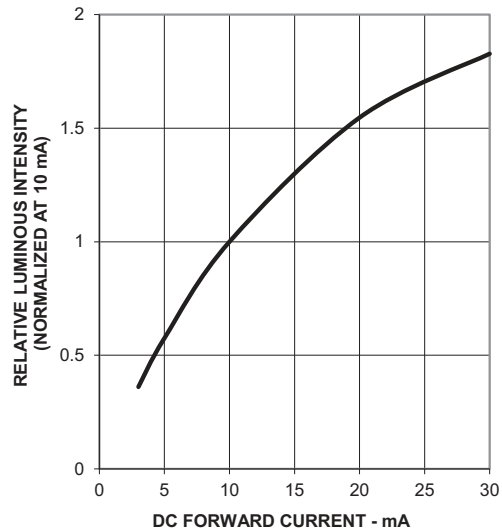
Figure 3: Relative Luminous Intensity vs. Forward Current
