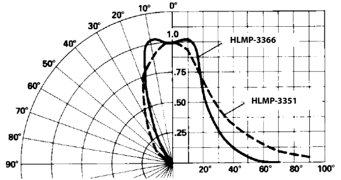
Figure 5: Relative Luminous Intensity vs. Angular Displacement
