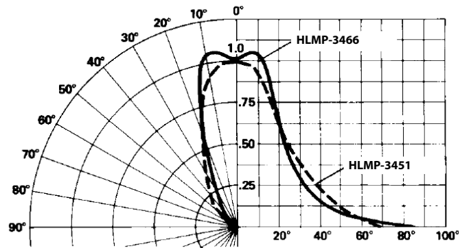
Figure 9: Relative Luminous Intensity vs. Angular Displacement
