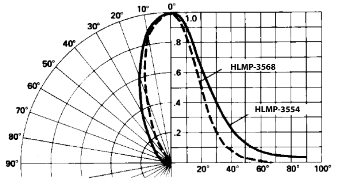
Figure 13: Relative Luminous Intensity vs. Angular Displacement
