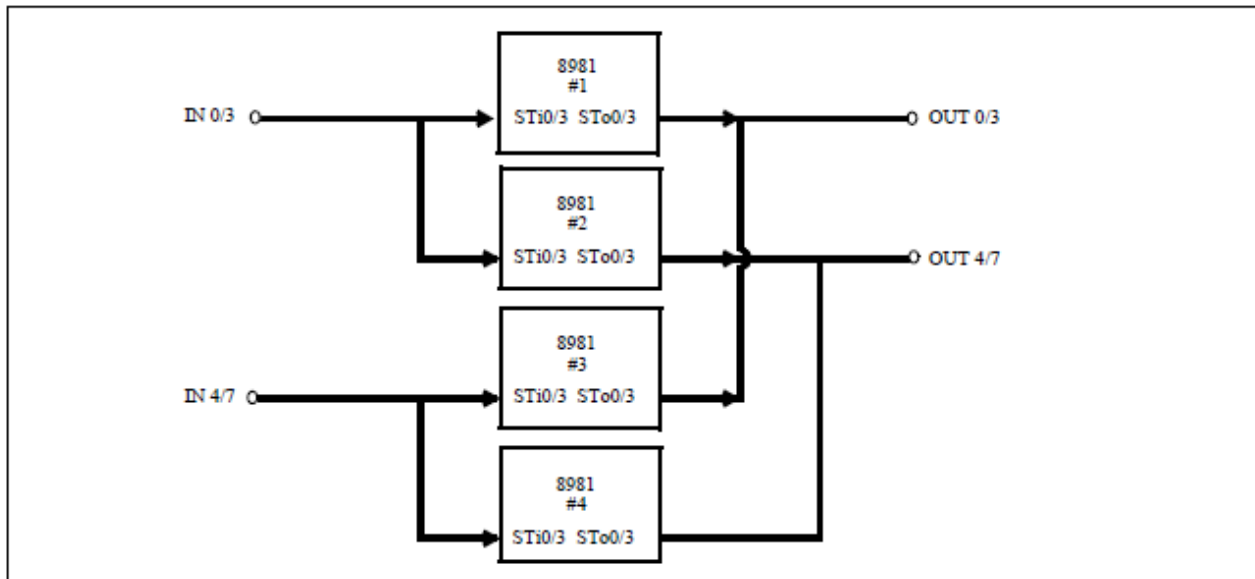
Figure 9 - Four 8981s Arranged in a Non-Blocking 16 x 16 Configuration
