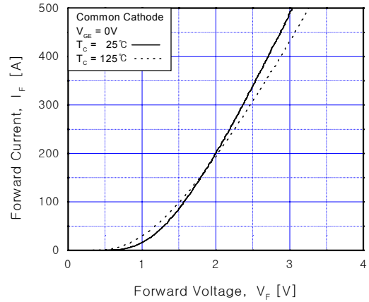
Fig 12. Forward Characteristics(diode)
