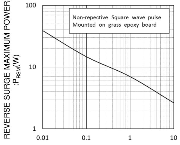
P_{RSM}-t CHARACTERISTICS
