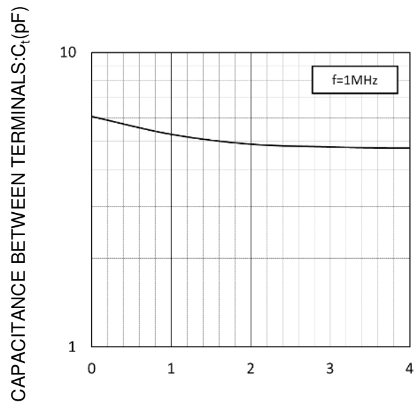
REVERSE VOLTAGE: V R (V) V R -C t CHARACTERISTICS
