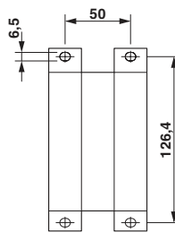
Dimensional drawing
