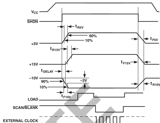
Figure 2. Power Sequence
