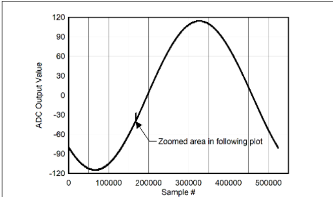
Figure 6-119. Background Calibration Core Transition (AC Signal)
