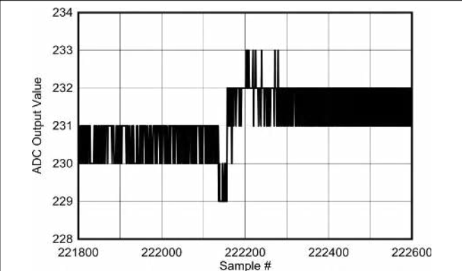
Figure 6-122. Background Calibration Core Transition (DC Signal Zoomed)
