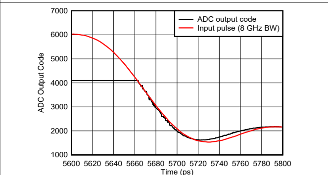
Figure 6-124. Pulse Overdrive Recovery Zoomed
