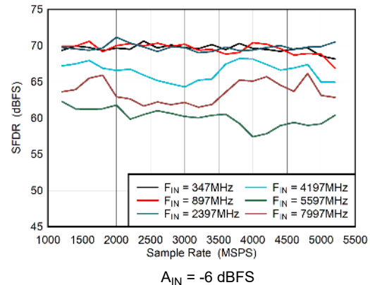
Figure 6-48. Dual Channel Mode: SFDR vs Sample Rate
