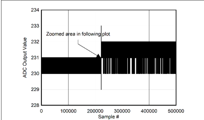
Figure 6-121. Background Calibration Core Transition (DC Signal)
