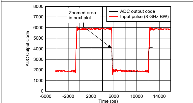
Figure 6-123. Pulse Overdrive Recovery
