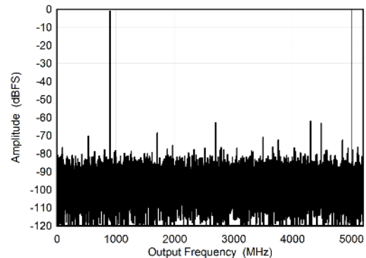
Figure 6-6. DES Mode: Single Tone FFT at 897 MHz
