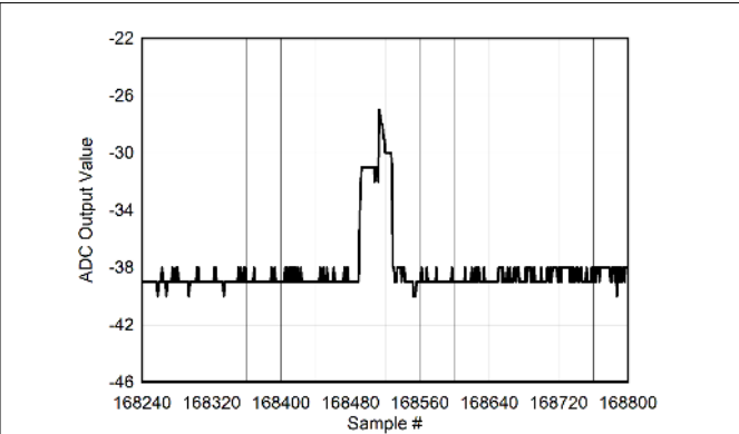
Figure 6-120. Background Calibration Core Transition (AC Signal Zoomed)
