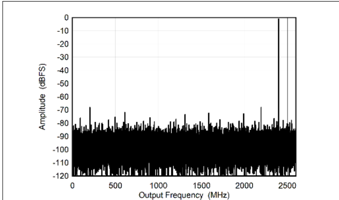
Figure 6-19. Dual Channel Mode: Single Tone FFT at 2397 MHz
