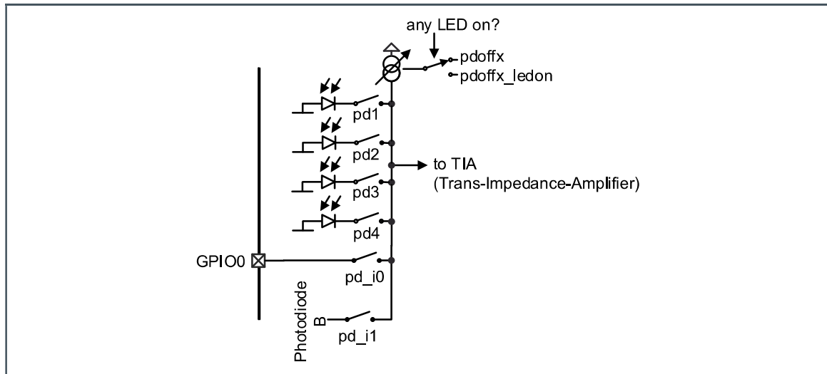
Figure 25: Photodiode Selection
