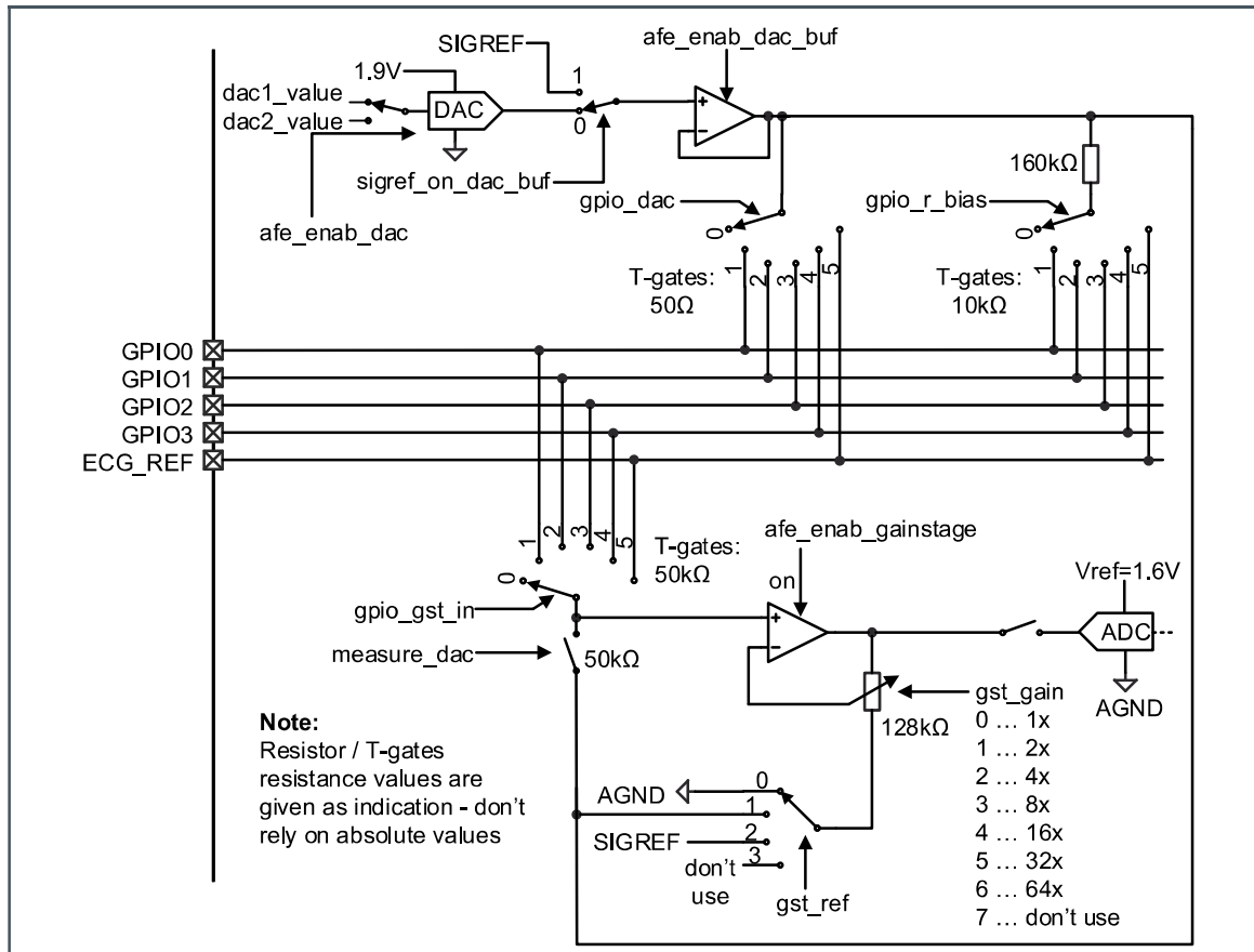
Figure 103: AFE Schematic
