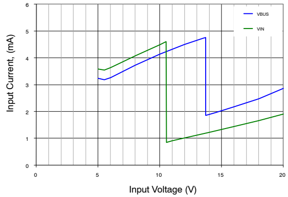
Figure 14. Quiescent Current vs. Input Voltage, I_{SYS} = 0\text{ A} , No Battery, LDO Off, NTC = GND, V_{BUSOVP} = 13.7\text{ V} , V_{INOVP} = 10.5\text{ V}
