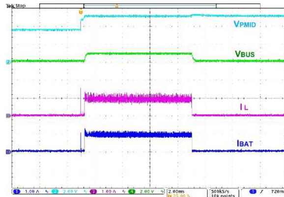
Figure 44. Boost Startup into V_{BUS} Fault
