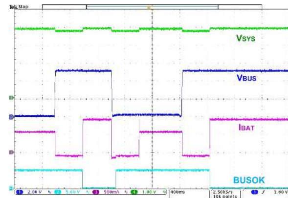
Figure 30. Input Source Selection, 5.0 V_{IN} Present, Insert/Remove 5.0 V_{BUS} , 3.8 V_{BAT} , 50 \Omega SYS Load
